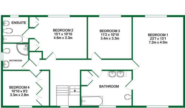
1ST FLOOR APPROX. FLOOR AREA 1053 SQ.FT. (97.9 SQ.M.)
