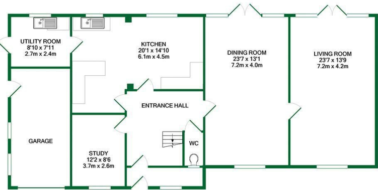
GROUND FLOOR APPROX. FLOOR AREA 1357 SQ.FT. (126.1 SQ.M.)
